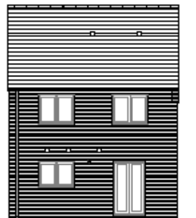
REAR ELEVATION
